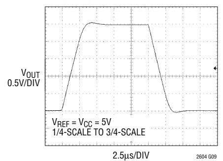
Large-Signal Settling
